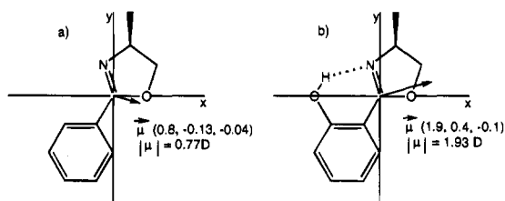
Figure 3. Dipole moments of the chosen models, (4S)-2-phenyl-4-methyloxazoline (a) and (4S)-2-(2'-hydroxyphenyl)-4-methyloxazoline (b), calculated by AM1 and drawn according to the physical convention.
